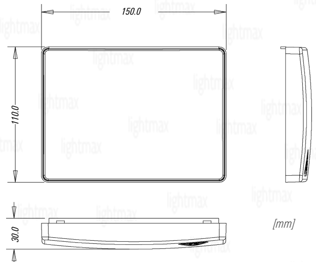
Structural Drawing
